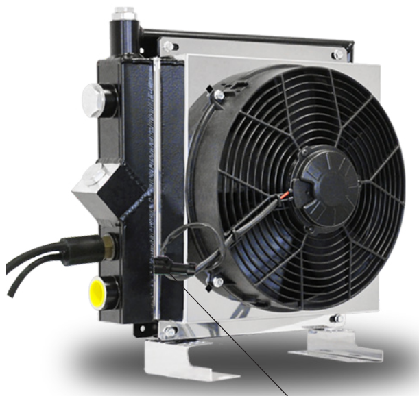
Scambiatore con by-pass Heat exchanger with by-pass
