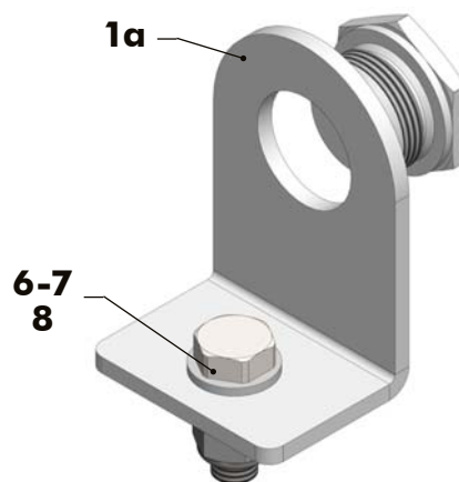
KIT SUPPORTO INNESTO RAPIDO ALETTE + TAPPO L-SHAPED BRACKET KIT FOR SINGLE QUICK COUPLING "WING TYPE" WITH PLUG 121-994-01501
