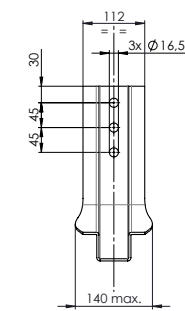
Dettaglio forature staffa Bracket holes detail
