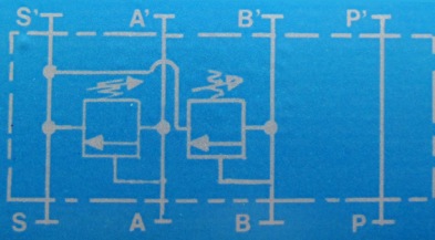
Schema idraulico Hydraulic scheme
