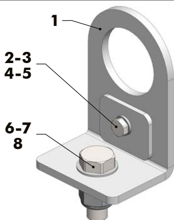
KIT SUPPORTO INNESTO RAPIDO ALETTE L-SHAPED BRACKET KIT FOR SINGLE QUICK COUPLING "WING TYPE" 121-994-00824
