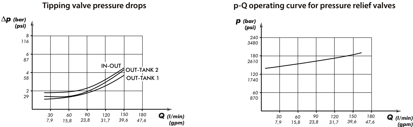
The graph refers to oil type ISO VG 46 a 50°
