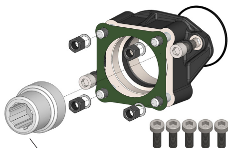
Mozzo / Hub 8x32x36 (ISO 14)
