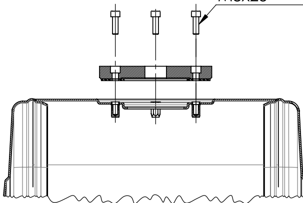
Serbatoi con flange imbuite e inserti filettati Tanks with dep-drawn flanges and threaded inserts
