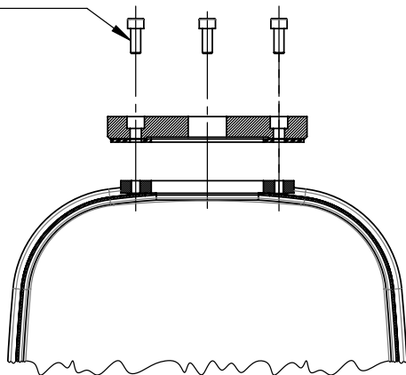
Serbatoi con flange saldate Tanks with welded flanges
