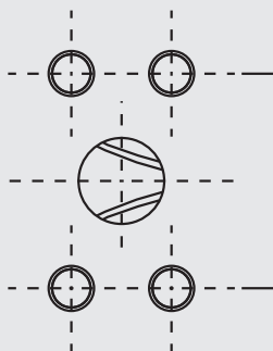
SAE 3000/6000
