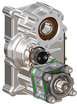
PTO series HIGH POWER for ZF TRAXON gearboxes.
