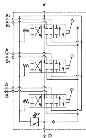
3 leve/levers
