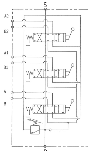
3 leve/levers
