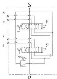
2 leve/levers
