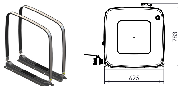
Montaggio retro-cabina Rear cab mounting
