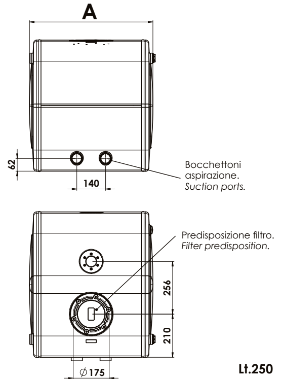
Montaggio retro-cabina Rear cab mounting
