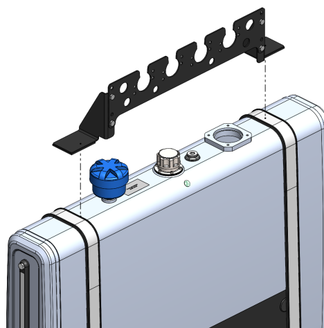
13590101227: Kit alto connessioni serbatoio Connection kit for top fitting
