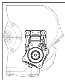
PTO Vertical ASSEMBLY - Low outlet
