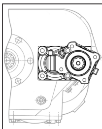
PTO Horizontal ASSEMBLY
