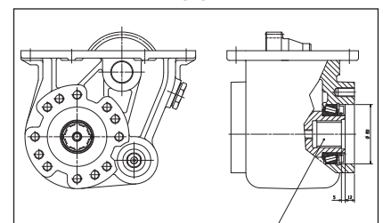
Female hub 8x32x36 (ISO14) Rear outlet
